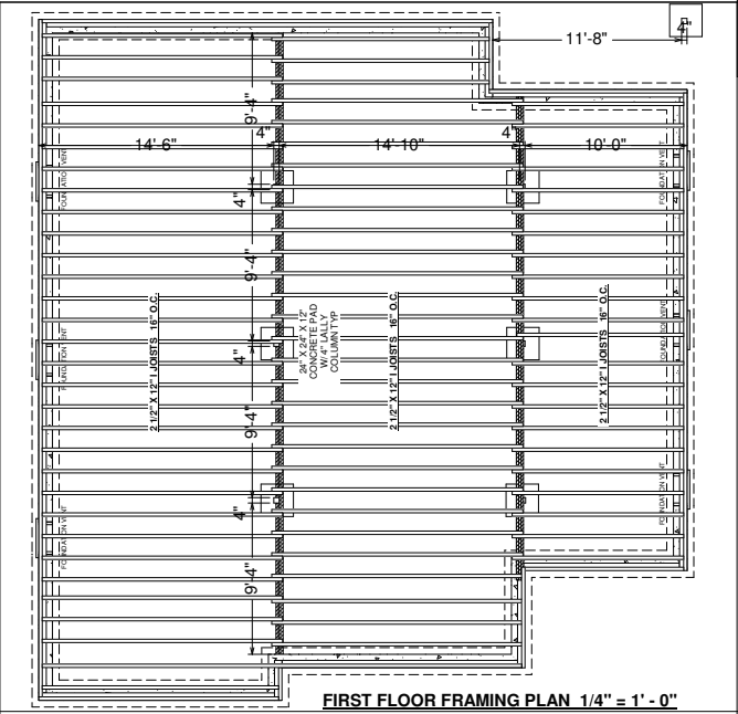
FIRST FLOOR FRAMING PLAN 1/4" = 1'-0"
