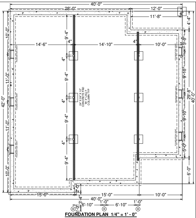
FOUNDATION PLAN 1/4" = 1'-0"
