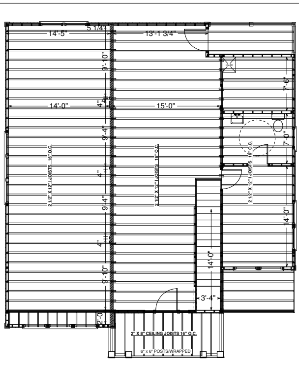
SECOND FLOOR FRAMING PLAN 1/4" = 1'-0"
