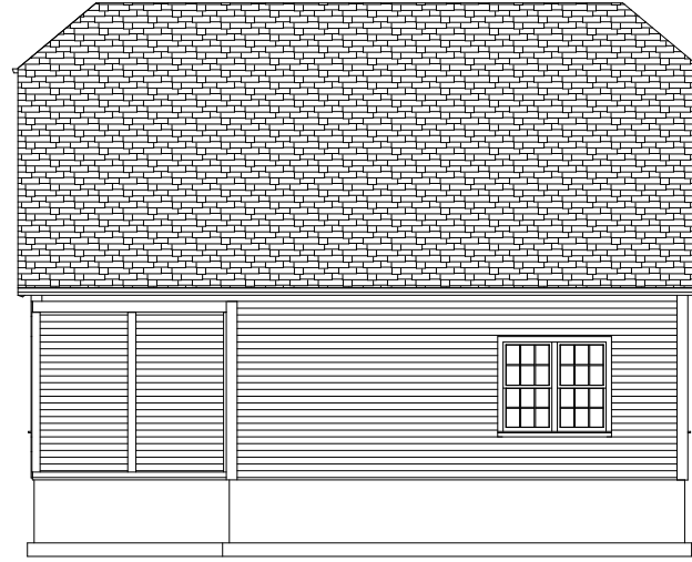
REAR ELEVATION 1/4" = 1' - 0"
